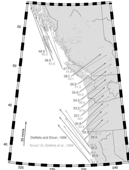
Figure 2. Comparison of relative plate motion velocities along the Cascadia margin. Light shaded arrows plot the azi-muth and magnitude of Pacific and Juan de Fuca plate motion relative to North America, as predicted by NUVEL-1A [DeMets et al., 1994], solid arrows from Table 1. The motion of the Juan de Fuca plate is constrained by magnetic lineations that record its motion relative to the Pacific plate. Thus changes in the Pacific–North America relative motion pole affect predicted Juan de Fuca–North America convergence. The new euler pole for Juan de Fuca–North America plate motion (Table 1) lies closer to the Juan de Fuca plate, and thus more rotation is implied, and the rate increases from south to north. A more northerly relative plate motion azimuth results in nearly or-thogonal convergence along the Canadian Cascadia margin. risks show volcanic vents associated with the continental arc. Modified from Pezzopane and Weldon [1993].
