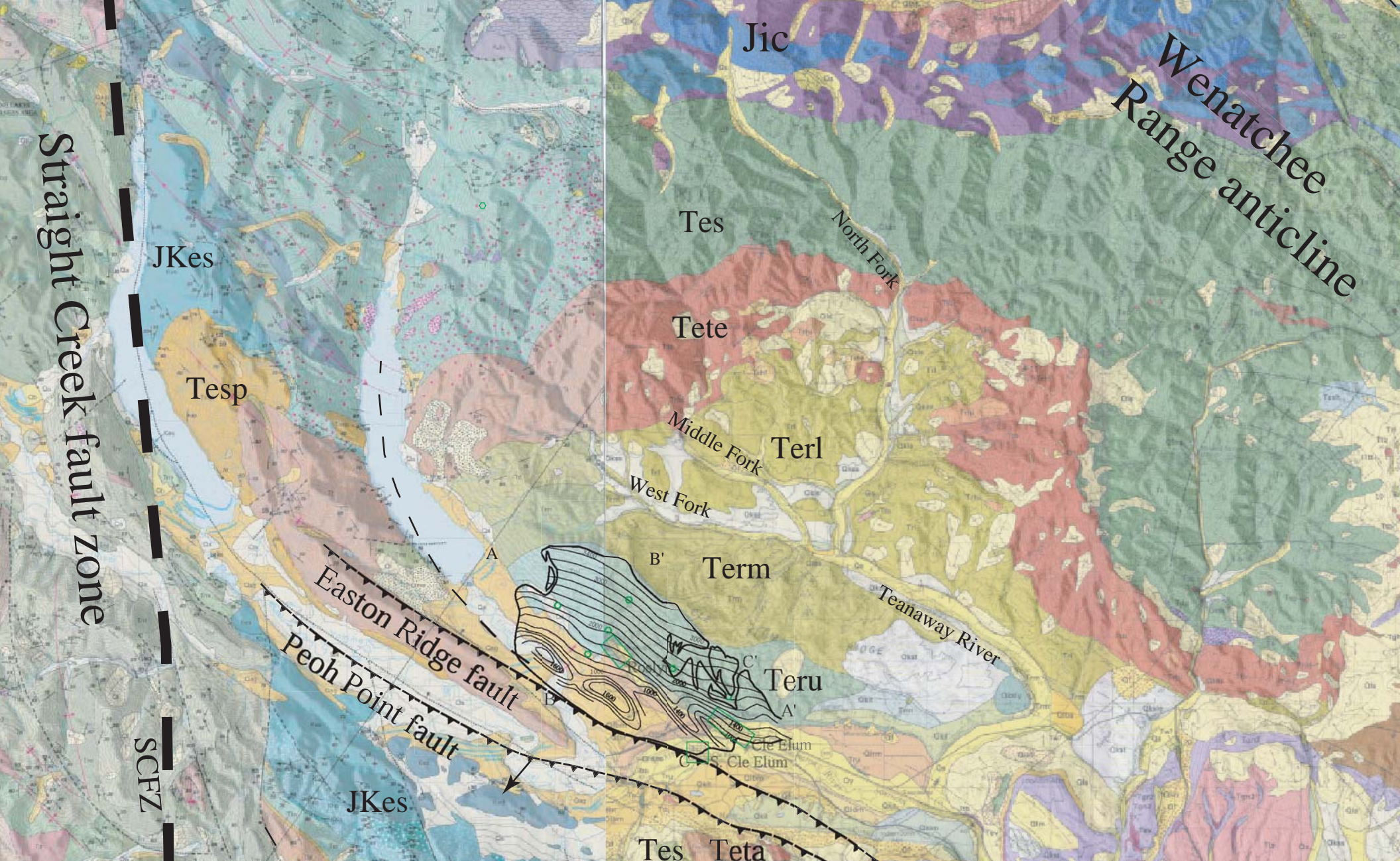
Figure 9. Structural contour map of Roslyn #5 coal seam (Shannon and Wilson, 1977, plate 3) overlain approximately on geology/topography (not to the highest cartographic standards). Note plunging folds associated with Easton Ridge fault, consistent with tectonic transport suggested by fault striations (arrow).
