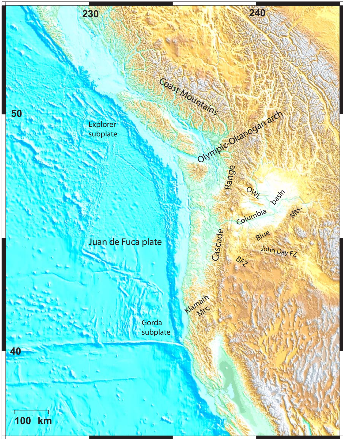
Figure 13. Physiography of the Cascadia margin and environs. Estimated bathymetry from Smith and Sandwell (1997); topography is GTOPO30.
