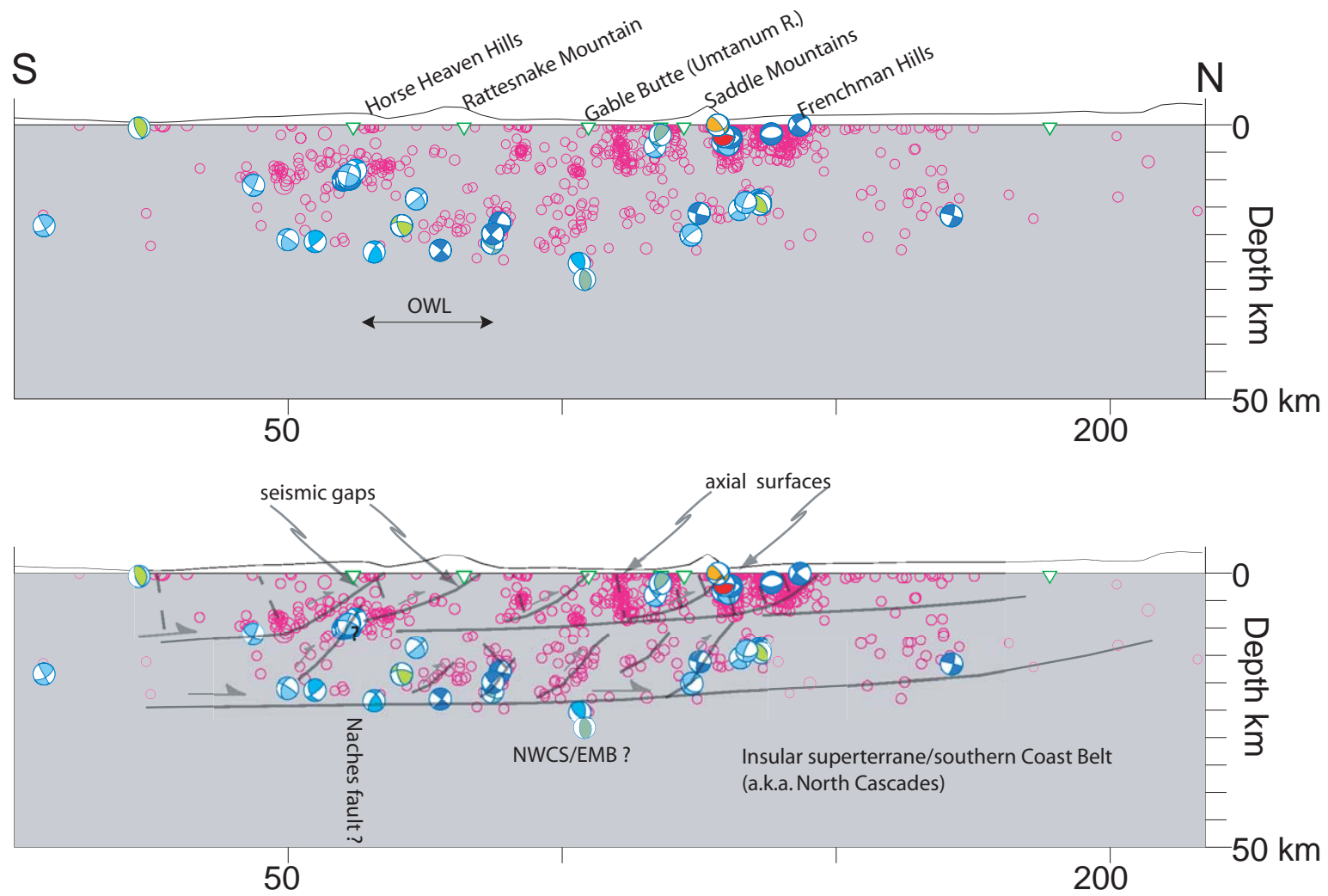
Figure 17. Profile 2 (see figure 16): data (top) and interpretation (bottom). Triangles are seismometer locations.
