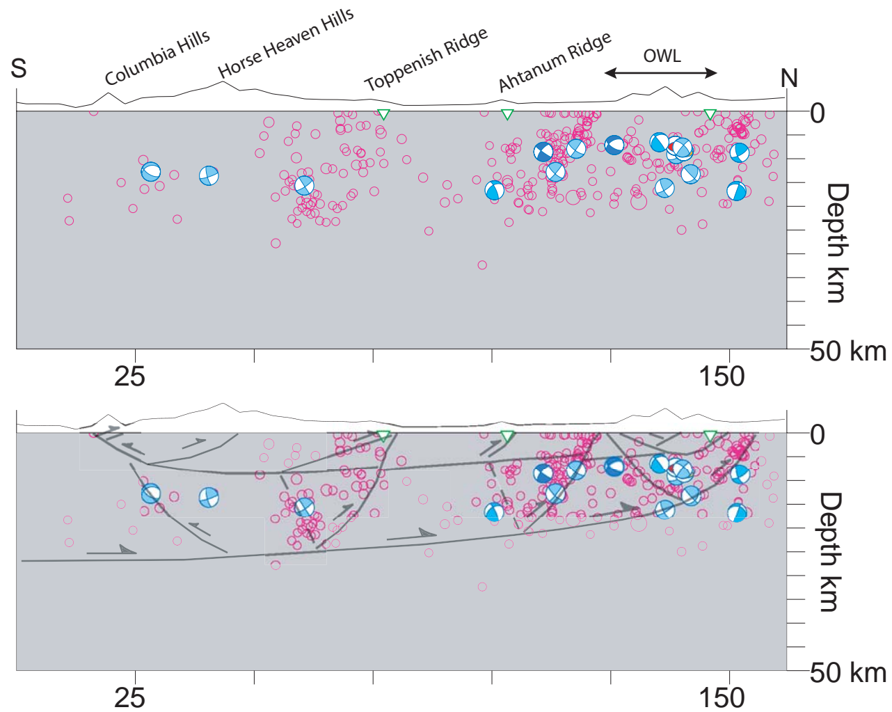
Figure 18. Profile 1: data (top) and interpretation (bottom). Deformation is basically thick-skinned, but the geometry of the shorter-wavelength folds seems to require decoupling at shallower levels as well.
