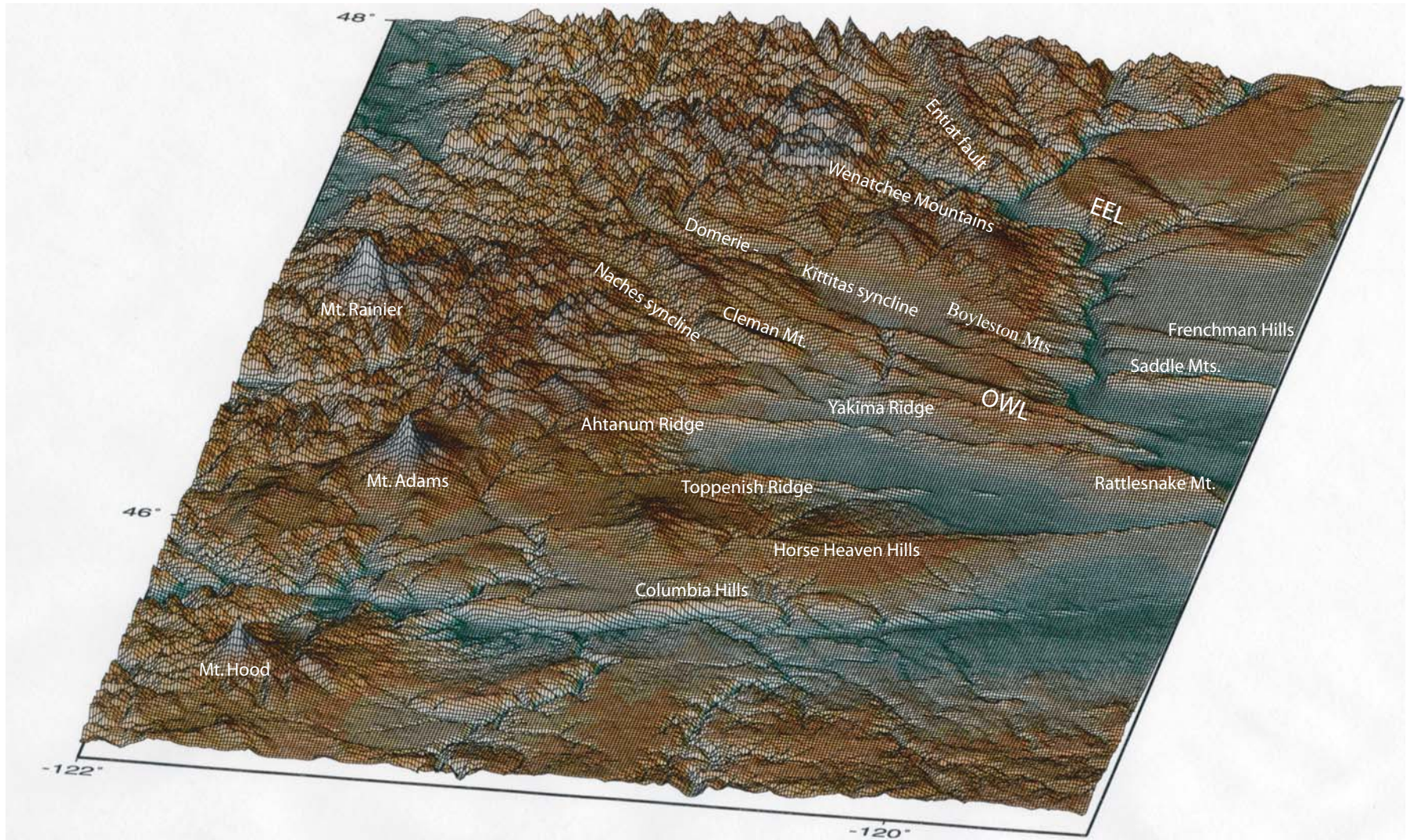
Figure 19. Oblique view of western Columbia Basin and adjacent Cascade Range. Relief greatly exaggerated.
