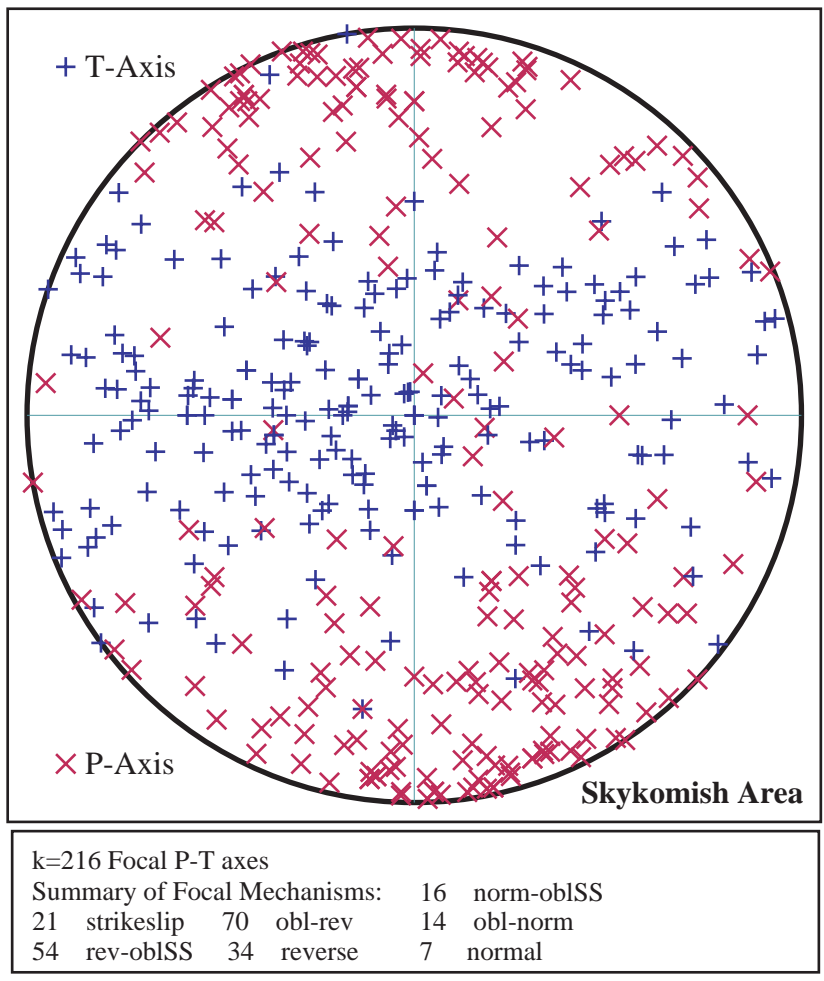
Figure 24. P- and T-axes from north of the Yakima fold belt. P-axes are concentrated slightly west of north. In the case of the Entiat area, they may be somewhat bimodal, with the secondary set directed NE-SW.
